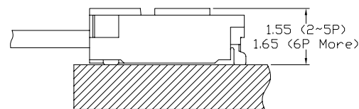
MATING VIEW
